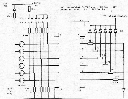
TYPICAL CIRCUIT
